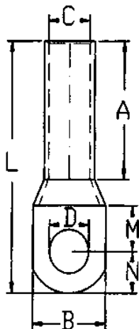
SOFT SLEEVES FOR TUBE TERMINALS COLOUR BLACK - TYPE P
